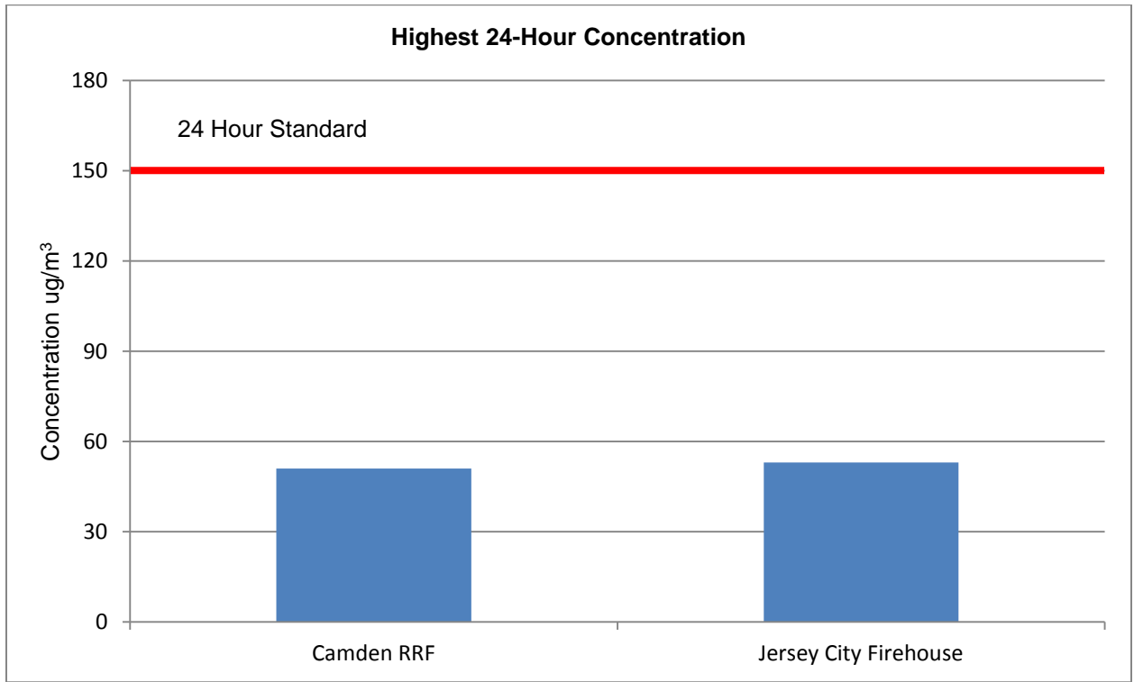
FIGURE 9B Summary of PM 10 Concentrations, New Jersey 2013
